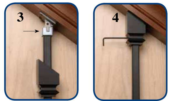
3 Snap Retaining Clip In Place
