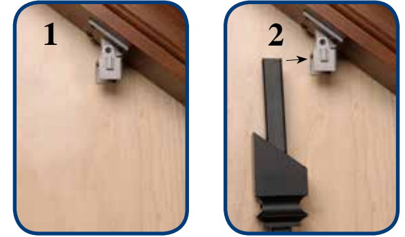
1 Install Clip To Handrail and Tread
