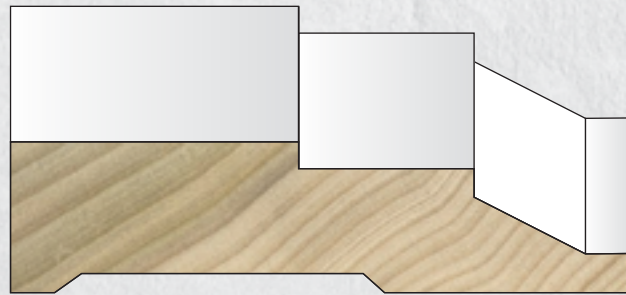
#8071 Bevel Casing 13/16" x 3-1/4" (FJ Poplar)
